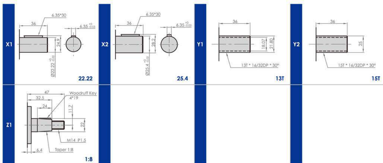
軸心尺寸 Dimension of Shaft (unit : mm)
