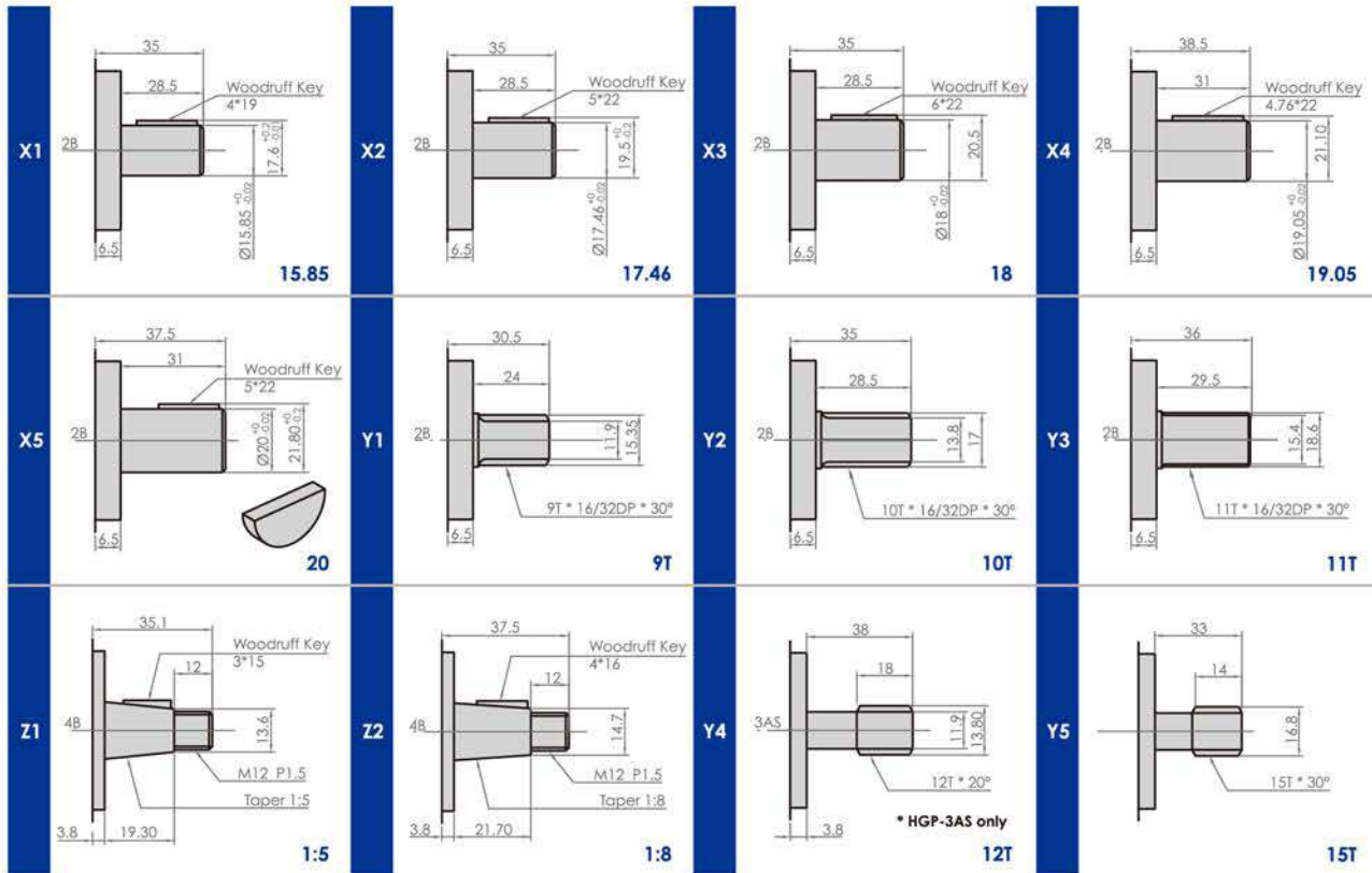
軸心尺寸 Dimension of Shaft (unit : mm)
